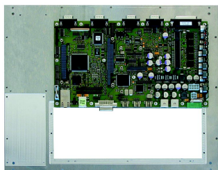
PIP mounted on customer supplied OEM cooling plate
